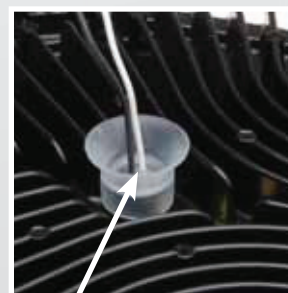
Wire entry seal to body
